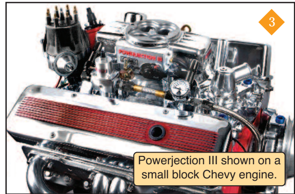
ABOVE - This is the POWERJECTION III on an engine. While the throttle body looks like a carburetor, it is actually a fully self contained throttle body that includes four port style injectors, fuel rails, idle air control, MAP sensor, and throttle position sensor.
